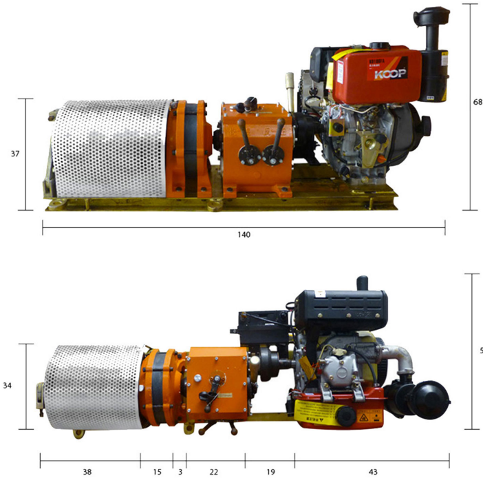
Dimensions in cms / Dimensiones en cms
